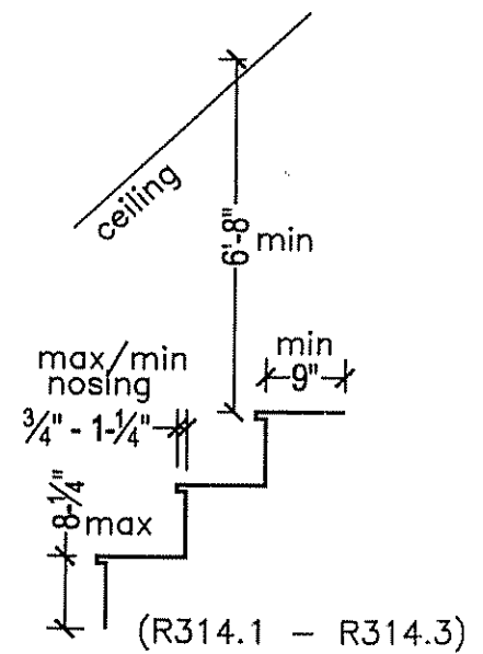
Stair Requirements
